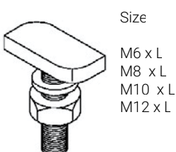
ZW 117 T - Bolt
