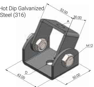
Universal Bracket
