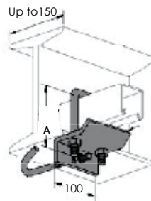
Beam Clamp
